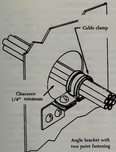
FIGURE 4-92. Cable clamp at bulkhead hole.
